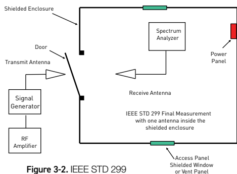
Figure 3-2. IEEE STD 299
